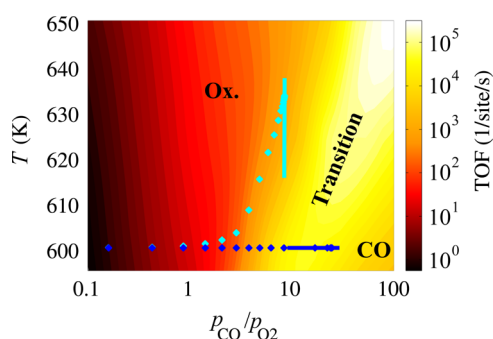
Figure 5. Intrinsic TOF-map for the CO oxidation at RuO 2 (110) 1p-kMC model as a function of the partial pressure ratio and temperature for constant total pressure of 5 bar. A rim of highest catalytic activity arises at the transition between an O-poisoned coverage (Ox.) regime in the upper left part of the shown range and a CO-poisoned coverage regime (CO) in the lower right part. Note the tilt of this rim toward higher p_{\text{CO}}/p_{\text{O}_2} ratios with increasing temperature, that is not obtained by a mean-field rate equation based microkinetic model (see text). Additionally marked with squares is the evolution of the gas-phase conditions at the center of the catalyst within the channel flow reactor after the switch to active feed for the isothermal (blue) and the adiabatic case (turquoise). The solid blue and turquoise lines further indicate the finally obtained range of gas-phase reaction conditions over the catalyst surface in the steady state for the isothermal and adiabatic cases, respectively.
