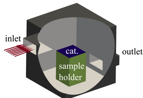
Figure 8. Representation of the reactor geometry considered as prototypical for in situ spectroscopic measurements of model catalysts. The gas enters with a uniform velocity at defined temperature at the inlet on the left, streams over the model catalyst surface (blue), and leaves the chamber through the outlet on the right. External heating allows us to control the temperature of catalyst and sample holder (green), while all remaining walls are set to adiabatic boundary conditions.
